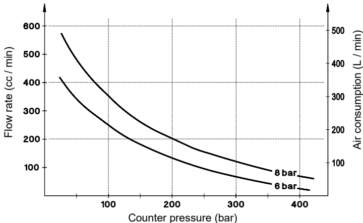
Performance chart: (Multi-purpose grease NLGI class 2 at ca. 20°C)
