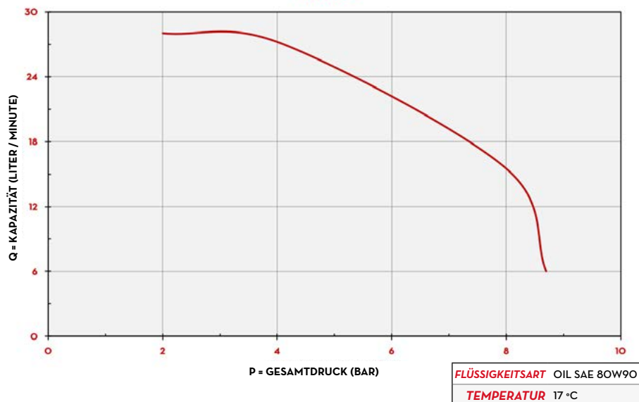
2-STUFIGE FILTRATION
