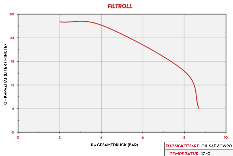
2-STUFIGE FILTRATION
