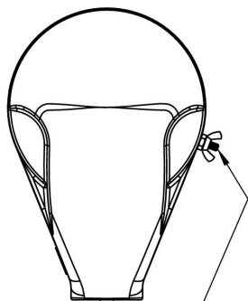
#10-32 GROUNDING STUD (Ø.19" (4.8mm))
