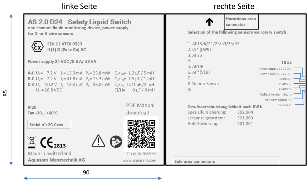
Abbildung 10 Typenschild AS 2.0 D24
