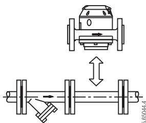
Meter with flanges
