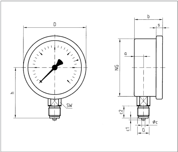
Dimensions (mm)
