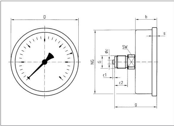
Dimensions (mm)
