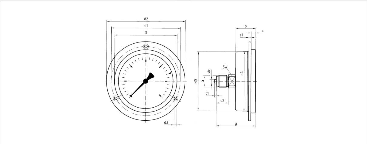
Dimensions (mm)
