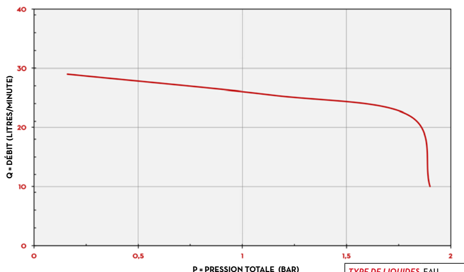
SB325_X PISTOLET
